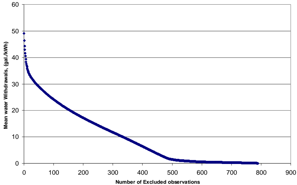
Figure V-4. The effect of excluding the highest values of unit water withdrawals use on the mean in the data for recirculating systems with cooling ponds or canals (Total n= 790)
